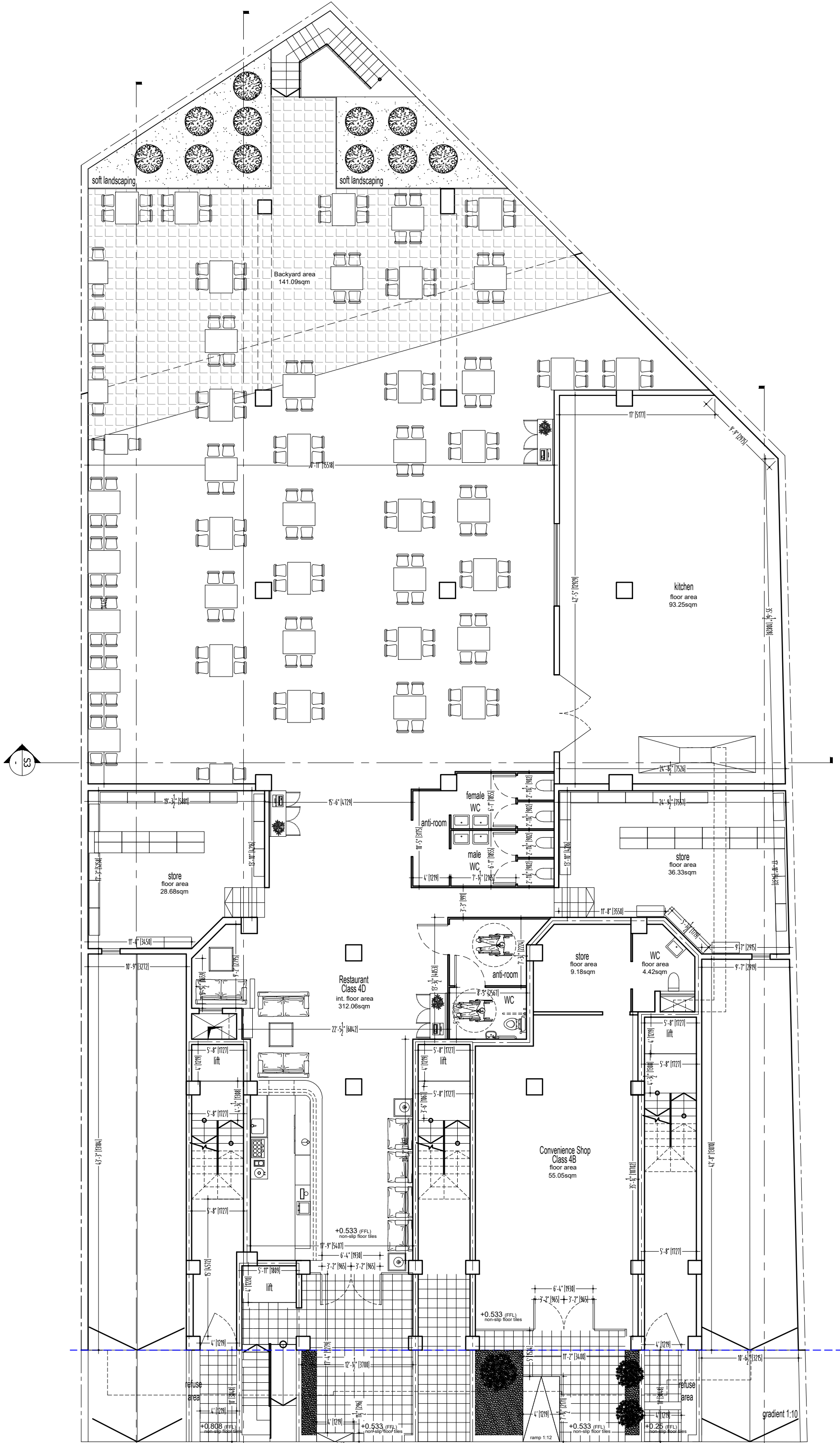
0 Ground floor level As Proposed Scale: 1:100
