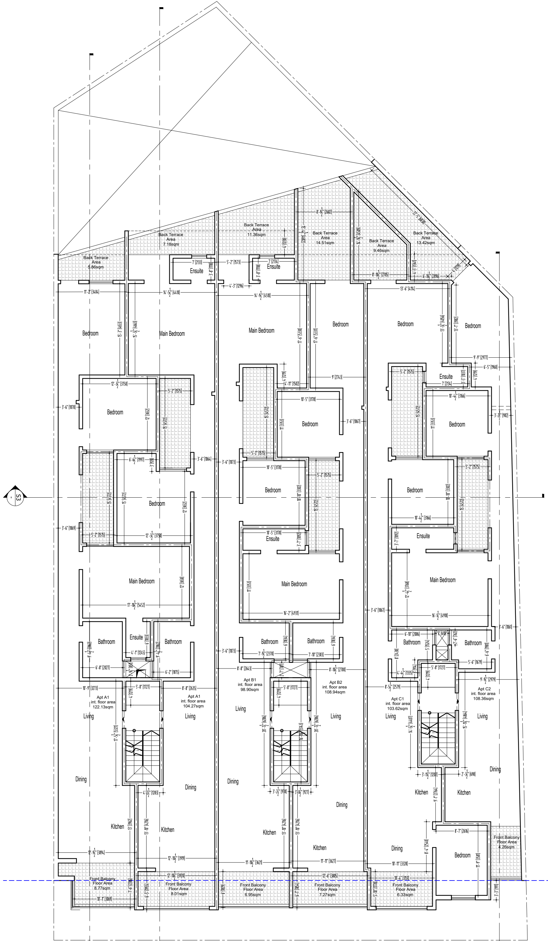
1 First floor level As Proposed Scale: 1:100
