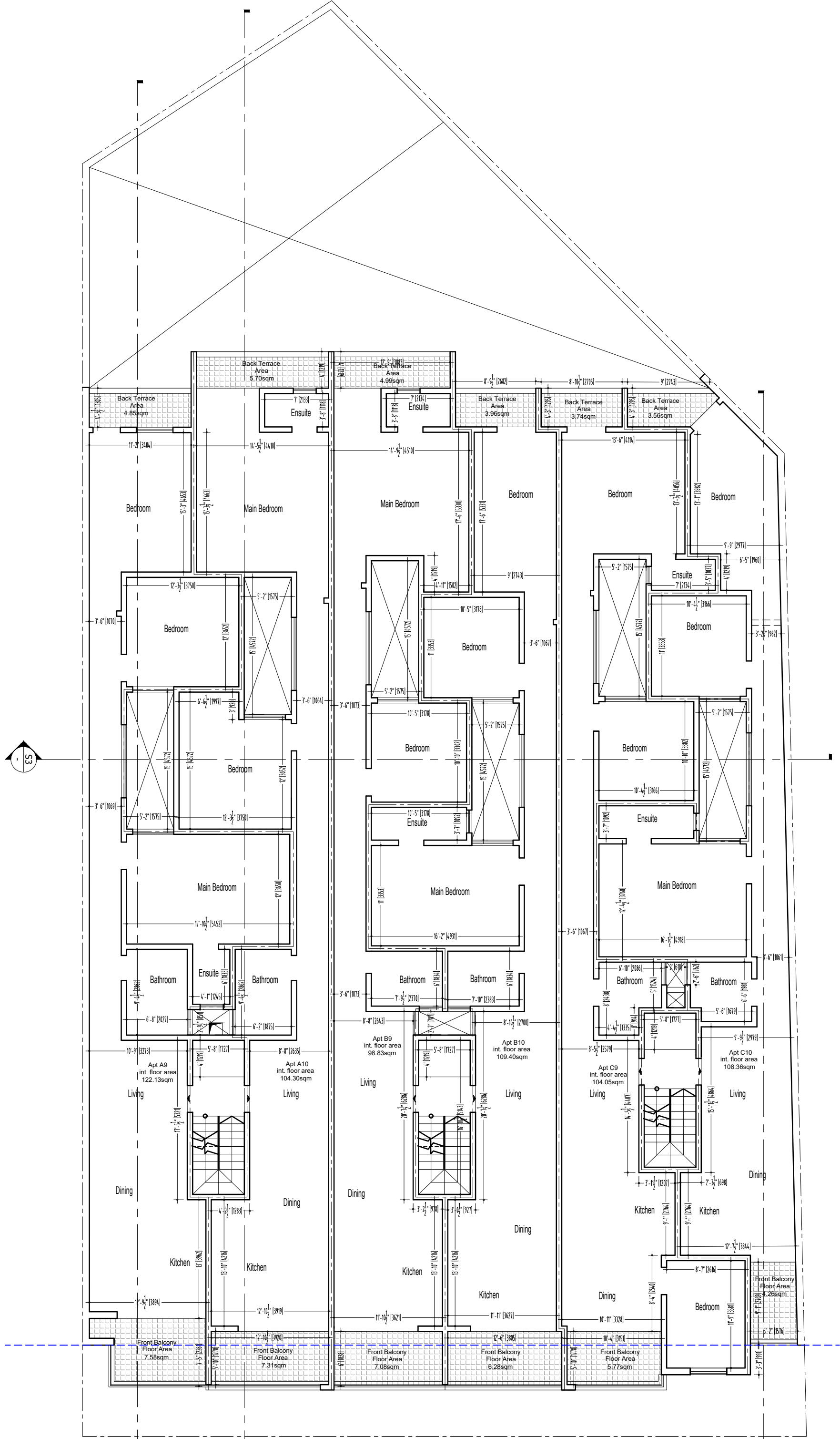
5 Fifth floor level As Proposed Scale: 1:100
