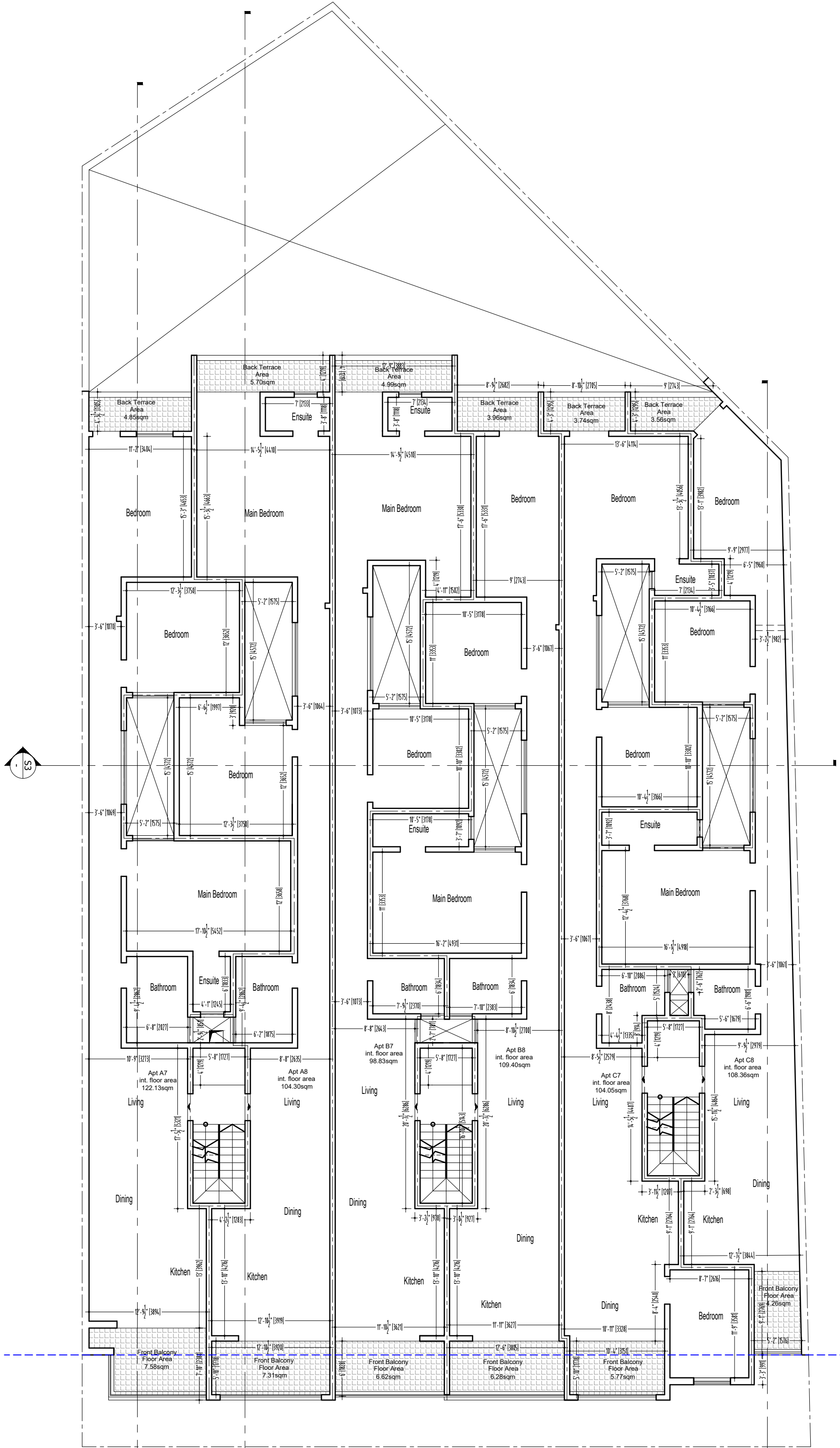
4 Fourth floor level As Proposed
