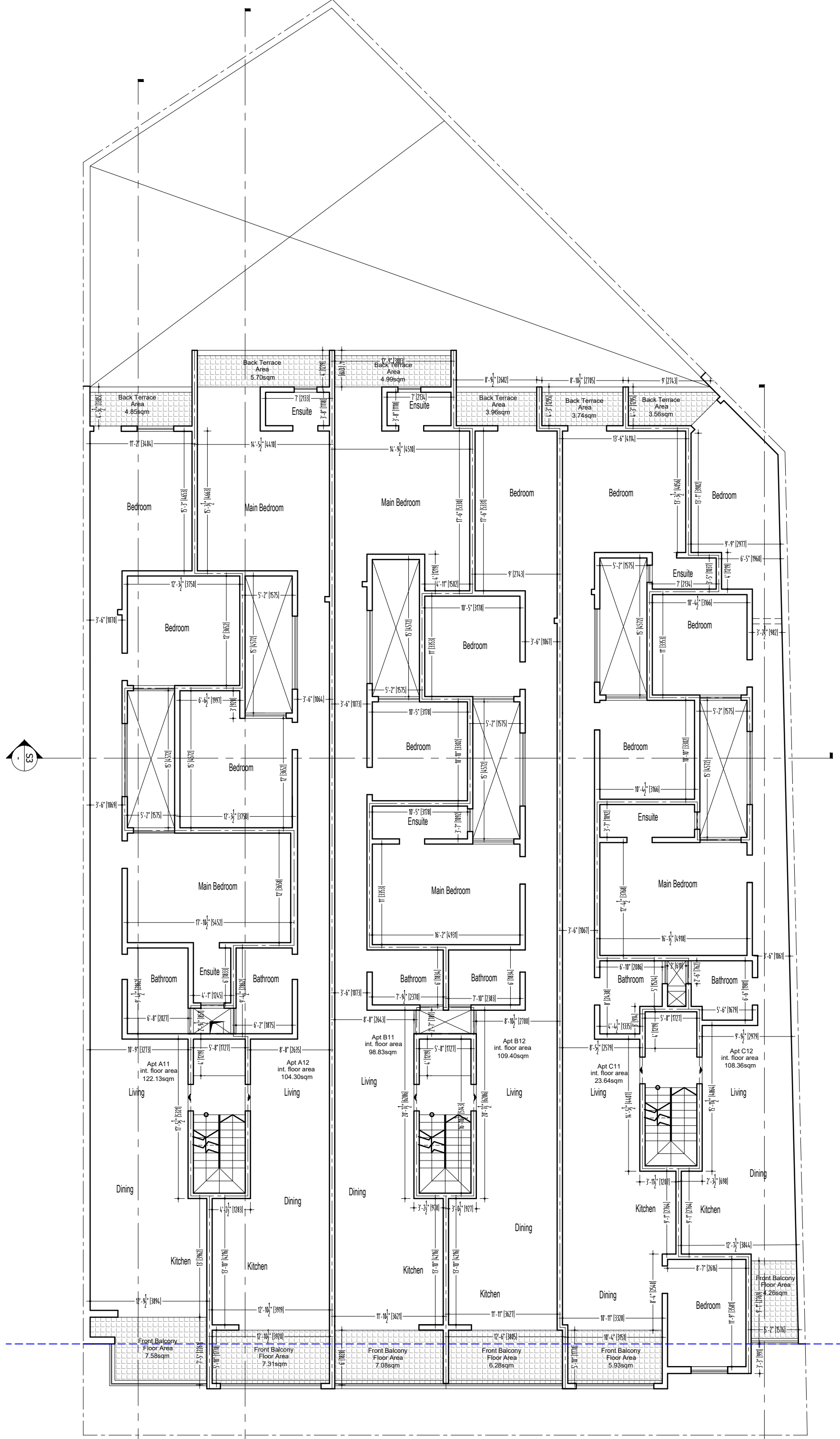
6 Sixth floor level As Proposed Scale: 1:100
