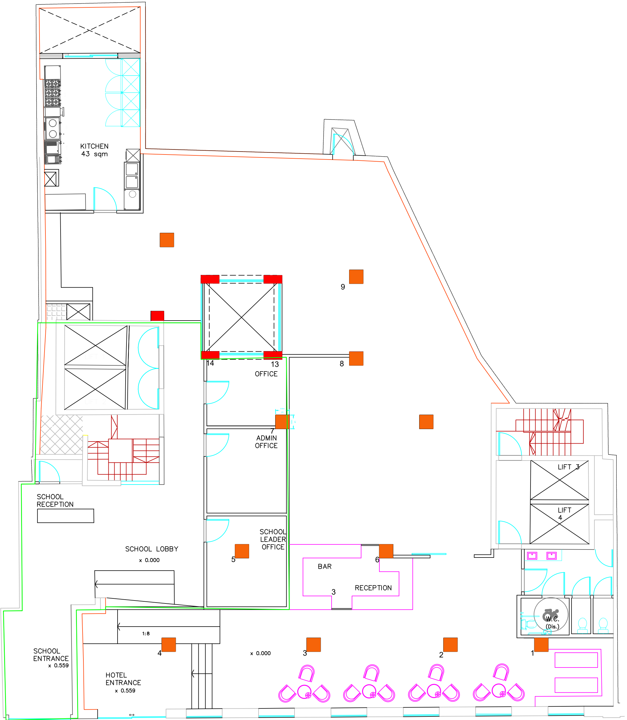
PROPOSED LEVEL 3 – School/ Hotel Reception SCALE 1:100
